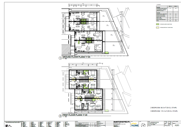
Figure 17: Proposed floor plans (17 – 2)
