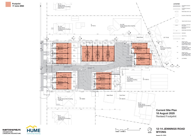
Figure 12: Proposed Site Plan
