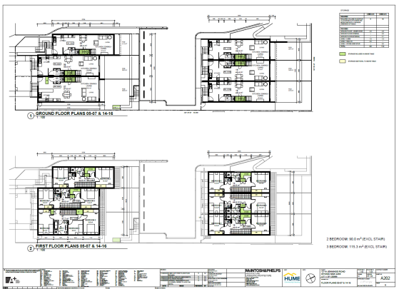
Figure 16: Proposed floor plans (5-7, 14-16)
