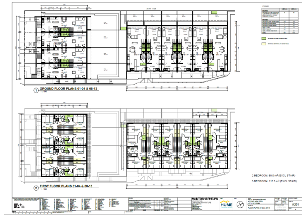
Figure 15: Proposed floor plans (1-4, 8-13)
